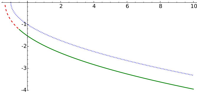
Figure 4.2. Graph of \Psi_{t,\rho} with a negative curvature
