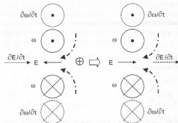
Fig. 3. The Faraday–Lenz law. Dashed lines represent \partial \omega / \partial t , and dash-dotted lines represent induced electric fields. The initial electric field generated by the positive ion is represented by solid lines, while the temporal change in the electric field due to the motion of the ion is represented by dashed lines
