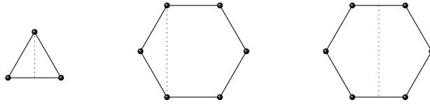
FIGURE 11. Walls in X
