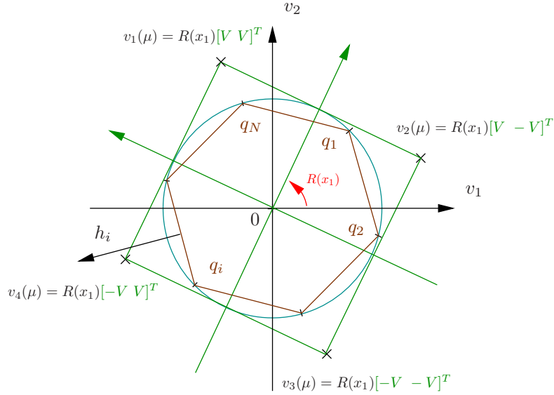
Fig. 2. Representation of control sets \mathcal{V}_{\mu u} for the system in the simulation example.
