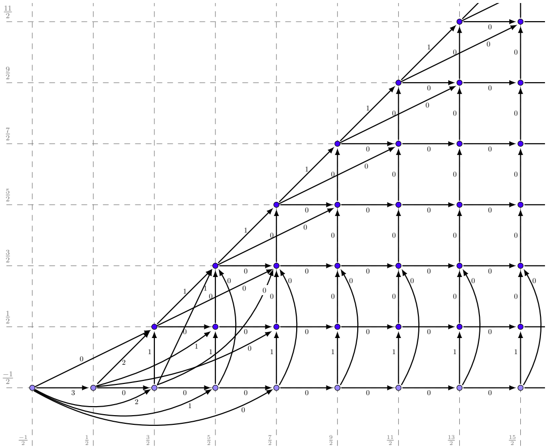
FIGURE 1. \mathfrak{osp}(5, 4)
