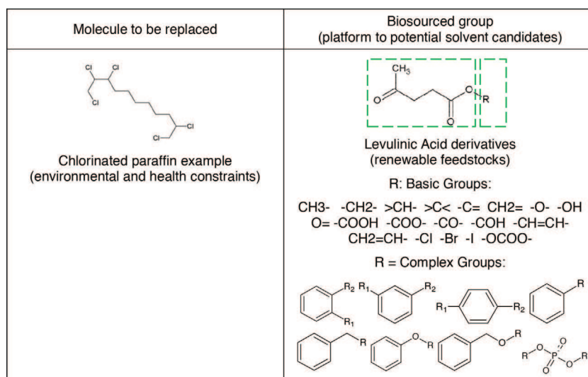
Fig. 10. A chlorinated paraffin example and building blocks used to generate alternative molecules.
