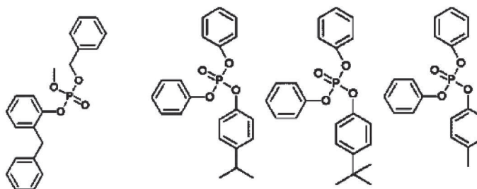
Fig. 11. Candidate and known alternatives for chlorinated paraffins (CP) substitution.
