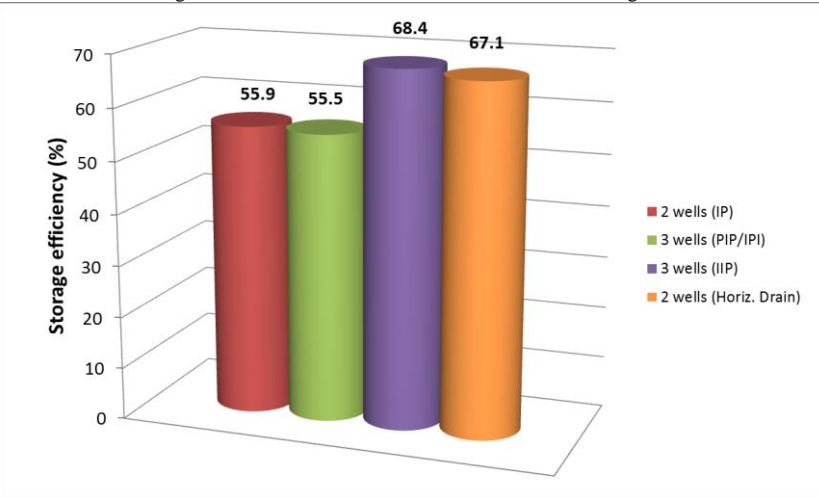
Fig. 14. Stored CO 2 efficiency for different wells configurations
