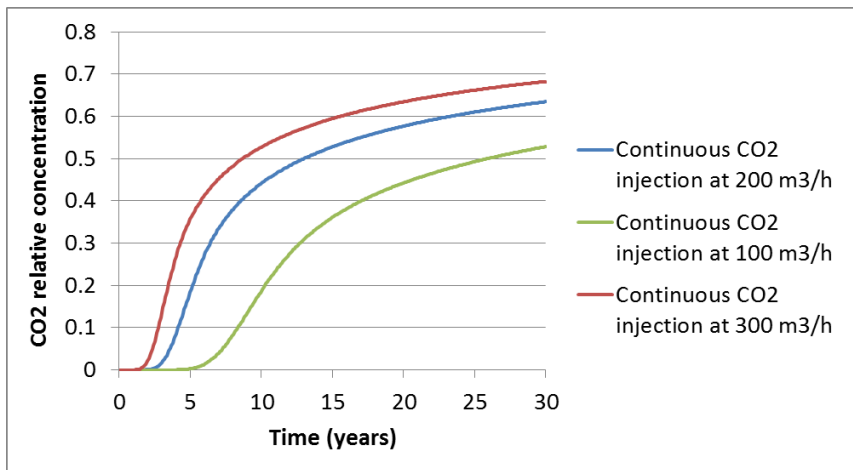
Fig. 2. CO 2 breakthrough at the production well for continuous injection at various flow rates. The injection and production well shoes are located 1.5 km apart (P2 in Fig 1).
