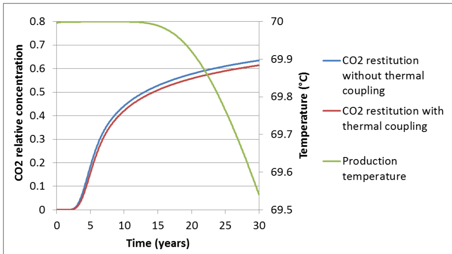
Fig 7. CO2 and thermal breakthrough at the production well for continuous injection
