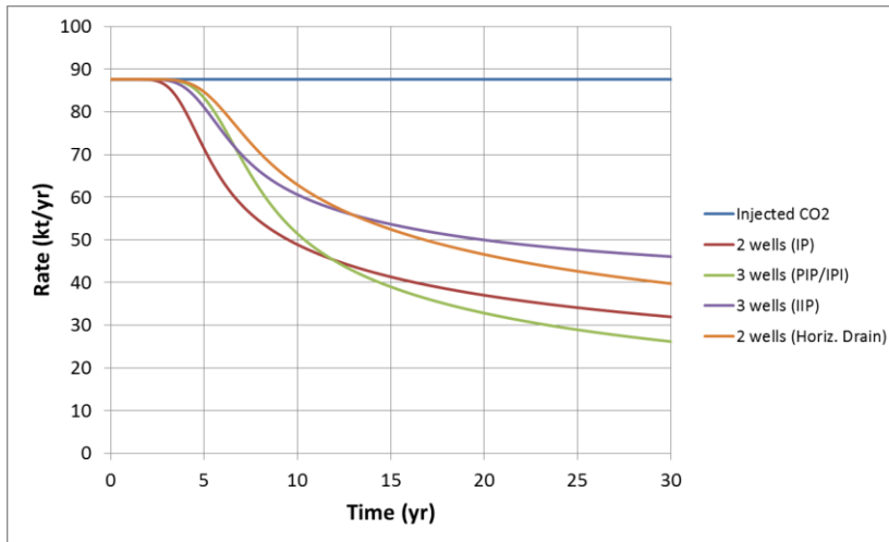
Fig. 12. Stored CO 2 rate for different wells configurations
