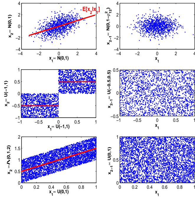
Figure 1: Scatterplots of x_2 versus x_1 for several joint distributions (on the left). Scatterplots of x_{2-1} , the sample of x_2 decorrelated from x_1 , versus x_1 (on the right).
