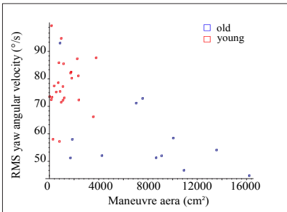
Fig. 19. RMS value of yaw angular velocity as a function of the manoeuvre area during the turn around phase (turn 2).
