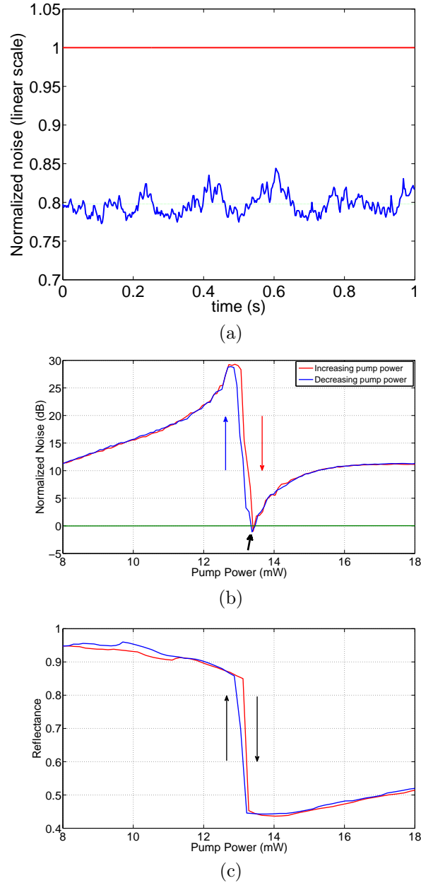
Figure 3: Intensity squeezing and bistability. (a) - Squeezed intensity noise at fixed pump power near the lower turning point (linear scale), on a 6\mu\text{m} pillar at cavity-exciton detuning of -5\text{meV} and a polariton-laser detuning of 0.19\text{meV} . The noise data were normalized with a measurement of the shot noise and a measurement of the dark noise, with S(t) = \frac{\text{noise}(t) - \langle \text{dark}(t) \rangle}{\langle \text{shotnoise}(t) \rangle - \langle \text{dark}(t) \rangle} ( \langle \dots \rangle is the time average). The measured noise reduction is 20.3 \pm 1.5\% (-1dB) below the shot noise limit before corrections, 35.8\% \pm 2.6\% after. The green line is the average noise and the red line is the shot noise. (b) - Intensity noise (spectral noise power, semi-logarithmic scale) as a function of the pump power for the same pillar under the same conditions as in (a). The noise increases smoothly toward a peak just before the bistability threshold, then suddenly drops to form a gap where intensity squeezing is observed, with about the same value as in (a). Here also the normalized spectral noise is obtained with 3 measurements (noise, shot noise and dark noise). In red is the curve obtained by increasing the pump power, in blue is the curve obtained by decreasing the pump power and the green line represents the shot noise (normalized to one). The thick black arrow points to where Fig.3 (a) was recorded. (c) - Bistability curve obtained by plotting the reflectance versus the pump power, for the same pillar under the same conditions as in (a) and (b). The color code is the same as in (b). Above the thresholds the transmission is increased, hence a sharp reduction on the reflectance.
