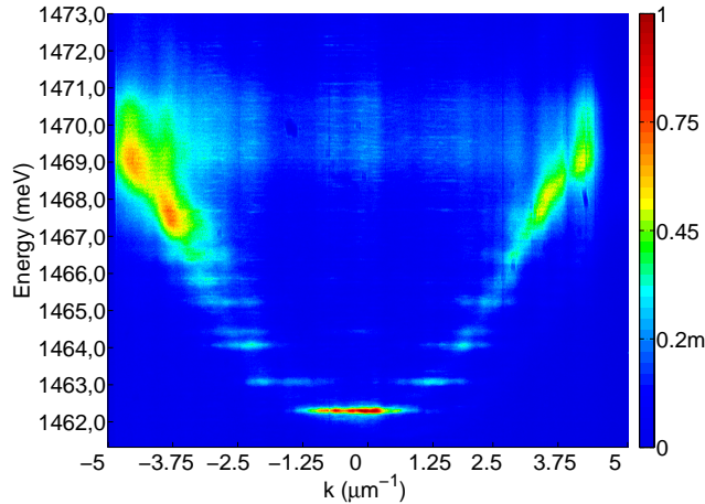
Figure 1: Energy modes separation. Dispersion curve for the 6\mu\text{m} circular pillar used in the experiment ( -5\text{meV} cavity detuning), obtained with a non-resonant pumping at 1550\text{meV} . The lower polariton branch with several spatial modes and the weakly excited upper branch are visible. The modes are energetically separated and squeezing is protected against multimode nonlinear coupling.
