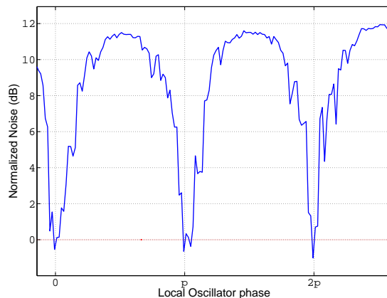
Figure 4: Homodyne detection. Experimental measurement of squeezing with homodyne detection for a pump-polariton detuning of 0.10\text{meV} on the same pillar as in Fig.3. The minima were verified to be in the amplitude quadrature. The squeezing obtained from the average between the values at 0, \pi and 2\pi is 14% before corrections and 27% after corrections. The reduced value of the squeezing here is mainly due to the non-optimal laser-polariton detuning.
