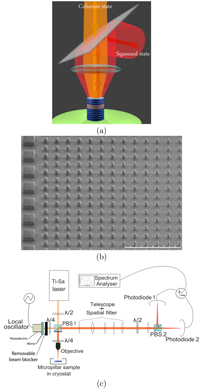
Figure 2: Sample and setup. (a) - Principle of squeezed light production with a pillar-shaped microcavity. The microcavity is made of a pair of quantum wells (white-red-white layers) sandwiched by two Bragg mirrors (alternation of light blue and dark blue layers); the green layer is the substrate. The orange beam represents the pump laser arriving on the sample at normal incidence, slightly blueshifted with respect to the energy of the lower polariton branch. The red beam represents the squeezed light emitted by the squeezed polariton field present in the microcavity. (b) - Image of the sample obtained with scanning electron microscopy. The different shapes and sizes of the pillars are visible. The scale bar corresponds to 100\mu\text{m} . (c) - Scheme of the experimental setup for the noise detection. The higher squeezing values were measured with the balanced detection setup, realized by blocking the local oscillator with the beam blocker. The choice of adding (+) or subtracting (-) the photodiodes signals determines the measurement: intensity noise (+) or shot noise (-). To measure the noise quadratures of the field one unblocks the local oscillator and set the mixer to (-); in this case the shot noise is measured by blocking the light reflected from the microcavity. PBS: polarizing beam splitter; \frac{\lambda}{2} , \frac{\lambda}{4} : half-wave, quarter-wave plate.
