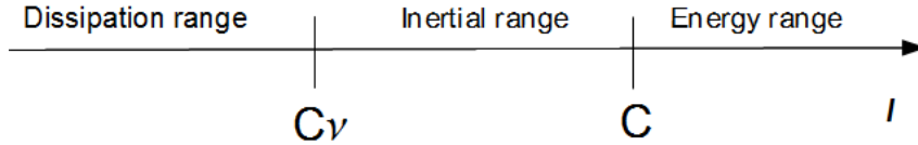
Figure 2: Scales for the 1D Burgers solutions
