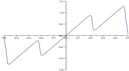
Figure 1: "Typical" solution of the Burgers equation
