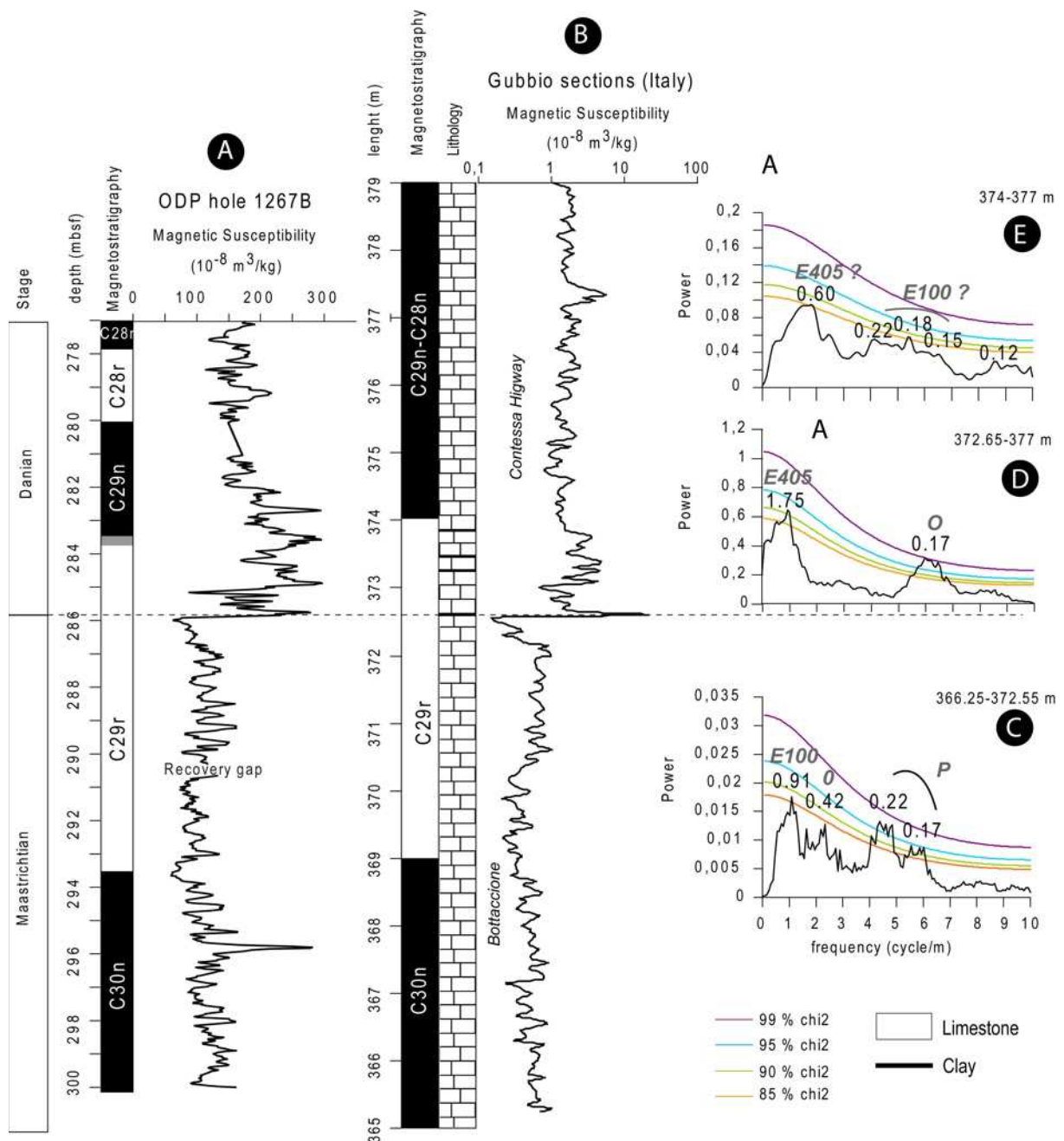
Figure 2: Cyclostratigraphic analysis of Magnetic Susceptibility variations from the Contessa Highway and the Bottaccione sections (Italy) on both sides of the Cretaceous-Paleogene boundary (B). Lithology of the Contessa Highway section for the C29r interval is from Coccioni et al. (2010). The MS signal from ODP Hole 1267B is also presented for comparison (A). The analysis method used was the multitaper method, completed by a Chi2 test to assess the reliability of the cycles detected. Comparison to MS variations from ODP Hole 1267B (South Atlantic) highlight a high similarity between the two signals. Precession and 100 kyr eccentricity variations are well defined in the Cretaceous, as highlighted by the spectral analysis of this interval (C), whereas the perturbations of the sedimentation rate following the K-PgB affect the record of the orbital parameters variations in the Paleogene. Results from the lowermost Paleogene spectral analysis (D) are very different from from analysis results of the C29n-C28n interval (E).
