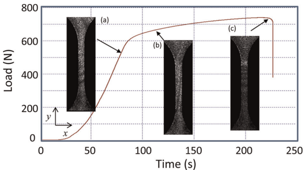
Fig. 6 Tensile experiment with Al alloy (2 per cent Mg) specimen. Pulling rate: 20 \mu\text{m/s} . The loading characteristic is shown along with typical interferometric fringe patterns observed: (a) prior to the yield point, (b) in the middle of the plastic regime, and (c) immediately before the fracture
