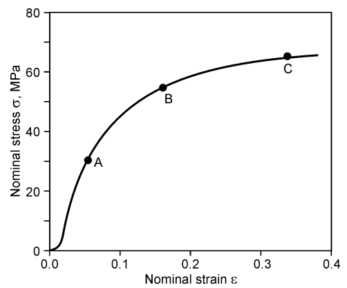
Fig. 1. Preload condition
