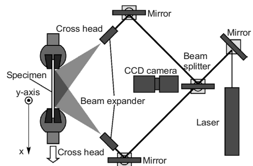
Fig. 2. Experimental arrangement
