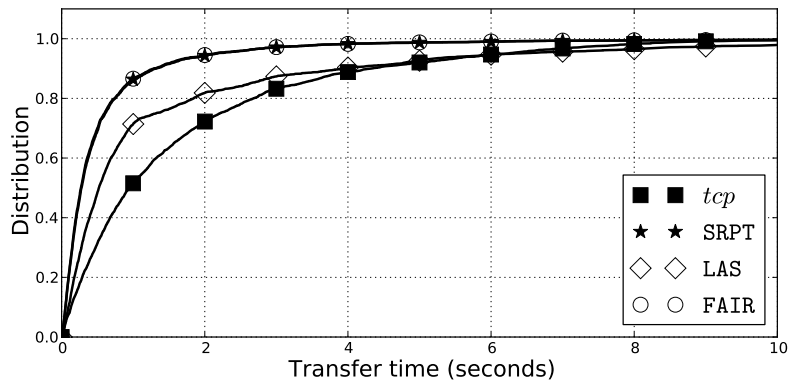
Figure 8: Distribution of flow transfer time with different scheduling policies.
