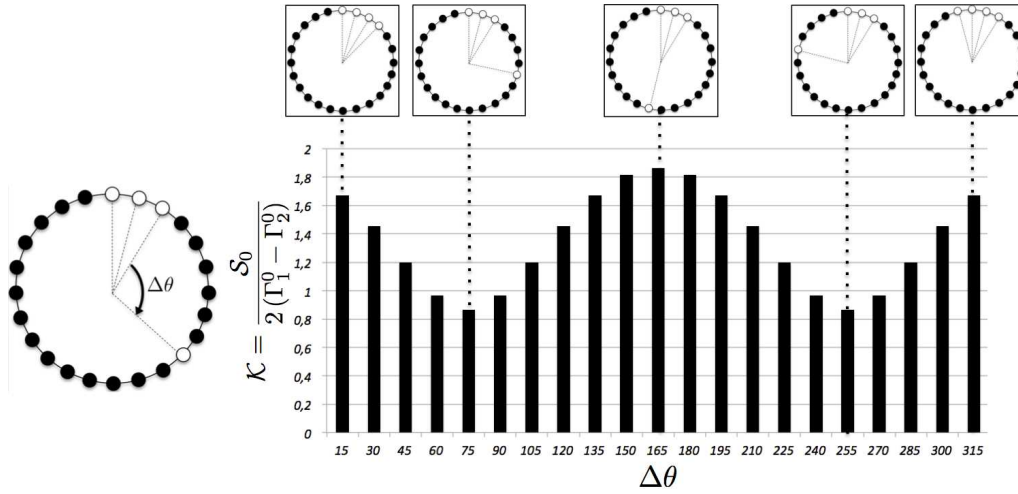
FIGURE 18. The reduced splitting strength ( \mathcal{K} ) for several patterns where three noCBO burners are kept together at the same place and the last noCBO burner's place is changed azimuthally. The splitting is then moderately affected by the asymmetry pattern.
