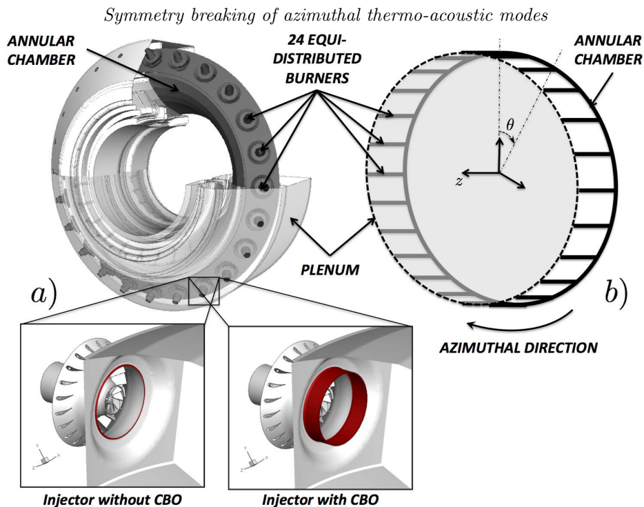
FIGURE 2. a) A typical 3D configuration of an industrial annular combustion chamber equipped with N = 24 burners with or without CBO and b) Network model of the annular chamber (—) with N = 24 burners. The annular plenum (---) is removed for the sake of simplicity.
