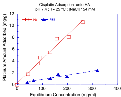
Figure 1. Adsorption isotherms of cisplatin onto hydroxyapatite (HA) in PB and PBS at 25 °C.
