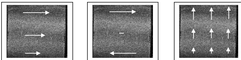
FIGURE 4. Sample interferograms with a horizontally sensitive ESPI setup (left two images) and a vertically sensitive ESPI setup (right image). Arrows represent displacement.
