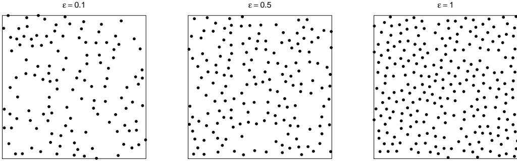
Figure 1: Typical realizations on [-1, 1]^2 of a Lennard-Jones model with parameters \beta = 100 , \sigma = 0.1 and \varepsilon = 0.1 (left), 0.5 (middle) and 1 (right).
