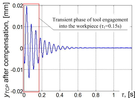
Fig. 15. Evolution of the dynamic displacement obtained after involving the error compensation technique into the analysis of robotic milling process
