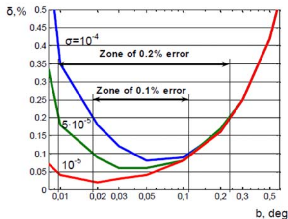
Figure 6.2 Identification errors for different amplitudes of the rotational deflections
