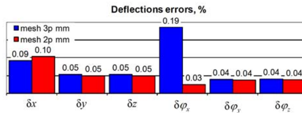
Figure 7.3 Influence of the stiffness matrix errors on the position accuracy
