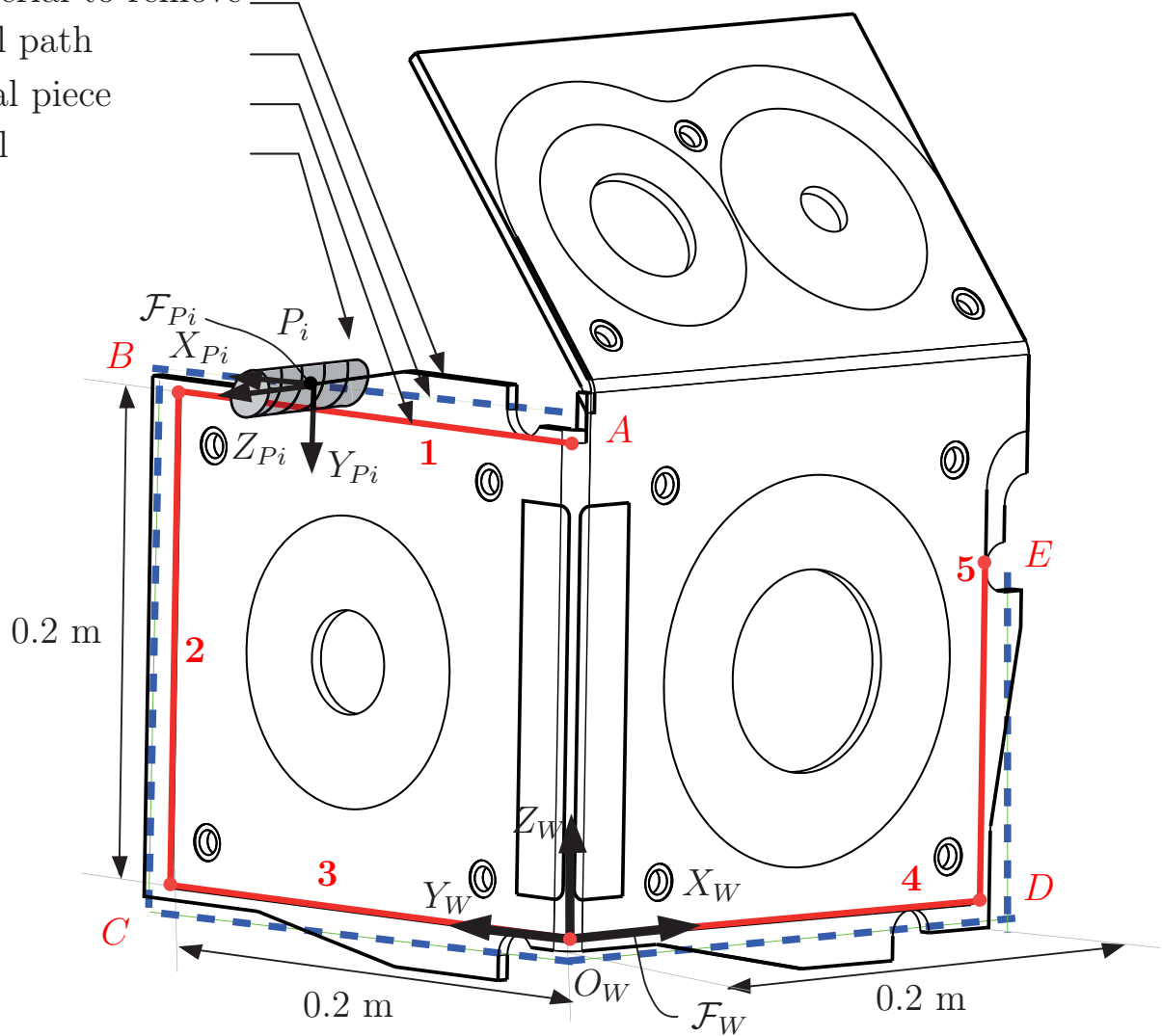
Figure 3.1 – Workpiece
