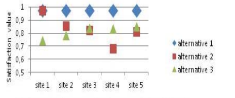
Fig. 6. Techno-Economic Objective
