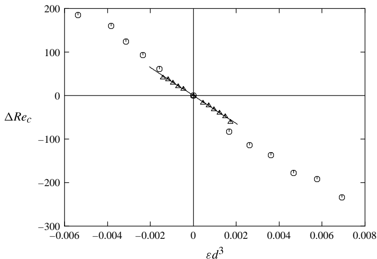
FIGURE 21. Predicted variation in the critical Reynolds number with \epsilon d^3 . The experimental values are shown by the triangles ( d_2 ) and circles ( d_3 ).
