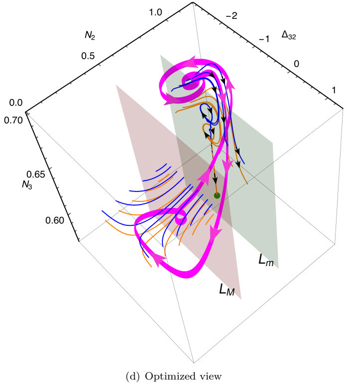
Figure 13: Example 2b. Parameters used: see Eq. (85), a = 0.5 and \lambda_\delta = 0.06 . Same caption as for Fig. 11. (c) and (d) Phase portraits of the desingularized super-slow subsystem (76) (shaded solid lines from orange to blue, only streamlines in the stable part of the CM are shown) compared to the trajectory of the full slow-flow system (49) (solid magenta lines) in the (\Delta_{32}, N_2, N_3) -space. Green disk marker indicates the position of the stable fixed point and arrows indicates the direction of the flow. The trajectory of full slow-flow system (49) is only plotted from t = 13000 s to the end ( t = 20000 s).
