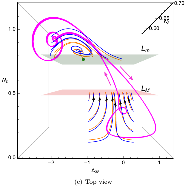
Figure 13: Example 2b. Parameters used: see Eq. (85), a = 0.5 and \lambda_\delta = 0.06 . Same caption as for Fig. 11. (c) and (d) Phase portraits of the desingularized super-slow subsystem (76) (shaded solid lines from orange to blue, only streamlines in the stable part of the CM are shown) compared to the trajectory of the full slow-flow system (49) (solid magenta lines) in the (\Delta_{32}, N_2, N_3) -space. Green disk marker indicates the position of the stable fixed point and arrows indicates the direction of the flow. The trajectory of full slow-flow system (49) is only plotted from t = 13000 s to the end ( t = 20000 s).
