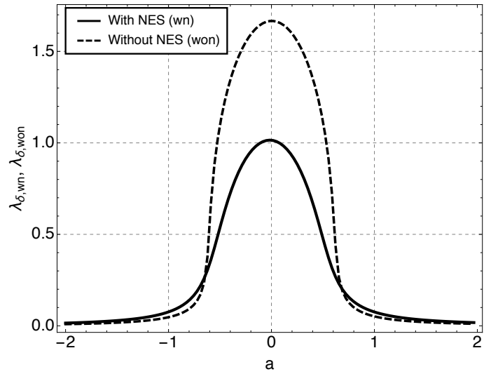
Figure 8: \lambda_{\delta, \text{wn}} and \lambda_{\delta, \text{won}} as a function of a . Parameters used: see Eq. (85).
