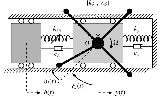
Figure 3: Descriptive diagram of the used helicopter system coupled to an ungrounded NES. View from the top.
