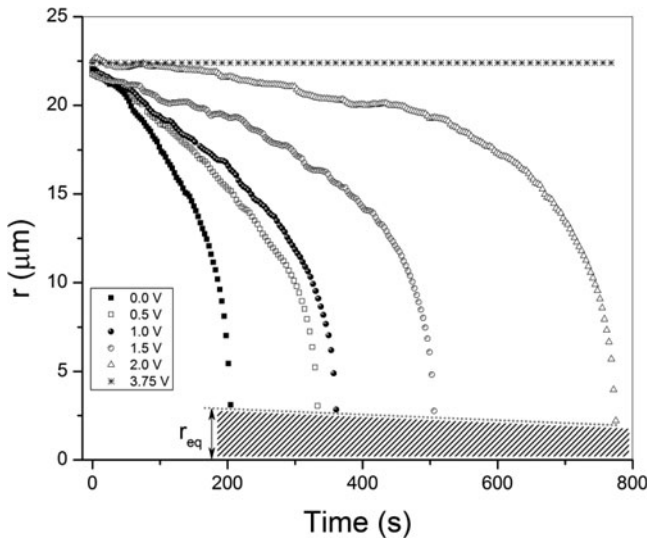
Figure 2. Position of the RC vs time during the optoelastic trapping for different values of the applied voltage. The initial position d_0 is 23 \mu\text{m} . The final value is the equilibrium distance r_{\text{eq}} from the centre of the trap.
