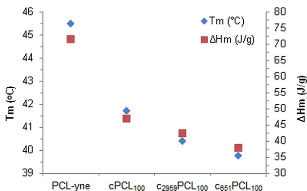
Fig. 4 Melting temperature and melting enthalpy (measured by DSC) of propargylated PCL and UV-crosslinked propargylated PCL with or without photoinitiator.
