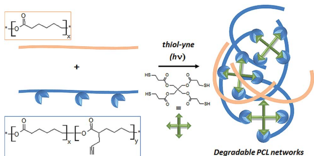
Scheme 2 Thiol-yne photo cross-linked PCL networks.
