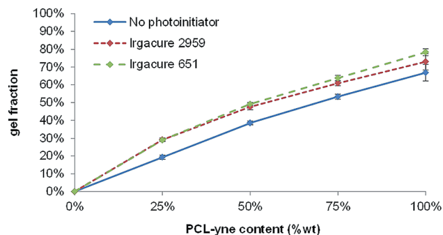
Fig. 1 Gel fraction of UV cross-linked PCL/propargylated PCL mixes with or without photoinitiator as a function of propargylated PCL content.
