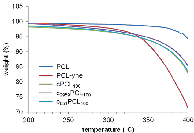
Fig. 3 TGA thermograms of non-modified PCL, propargylated PCL and UV cross-linked propargylated PCL with or without photoinitiator.
