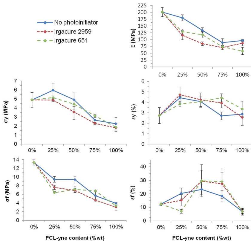
Fig. 5 Mechanical tensile properties of UV cross-linked PCL/propargylated PCL mixes with or without photoinitiator as a function of propargylated PCL content.
