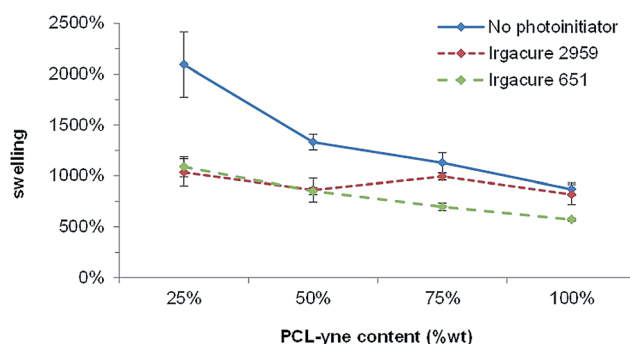
Fig. 2 Swelling of UV cross-linked PCL/propargylated PCL mixes with or without photoinitiator as a function of propargylated PCL content.
