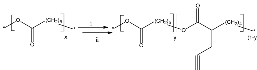
Scheme 1 General reaction scheme for the synthesis of propargylated PCL (PCL- yne ) with (i) LDA (0.5 eq. per CL unit), -50^\circ\text{C} , 30 min and (ii) propargyl bromide (0.5 eq. per CL unit), -30^\circ\text{C} , 30 min.
