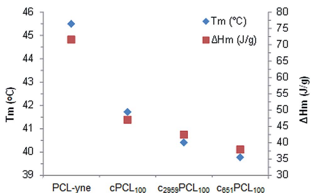
Fig. 4 Melting temperature and melting enthalpy (measured by DSC) of propargylated PCL and UV-crosslinked propargylated PCL with or without photoinitiator.
