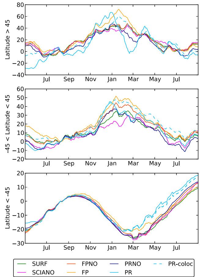
Figure 6. Average seasonal cycle for three latitudinal bands. Model-simulated mixing-ratio fields are evaluated at locations of surface sites used in the SURF inversion. Ten-day moving average is applied to remove the short-term variability.
