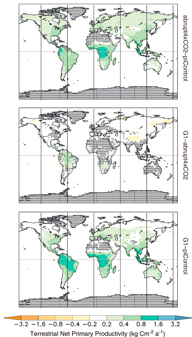
Figure 9. All-model ensemble annual average differences in terrestrial net primary productivity ( \text{kg C m}^{-2} \text{ a}^{-1} ), averaged over years 11–50 of the simulation. Top panel shows abrupt4xCO2 – piControl , middle panel shows G1 – abrupt4xCO2 , and bottom panel shows G1 – piControl . Stippling indicates where fewer than 75% of the models (for this variable, 6 out of 8) agree on the sign of the difference.
