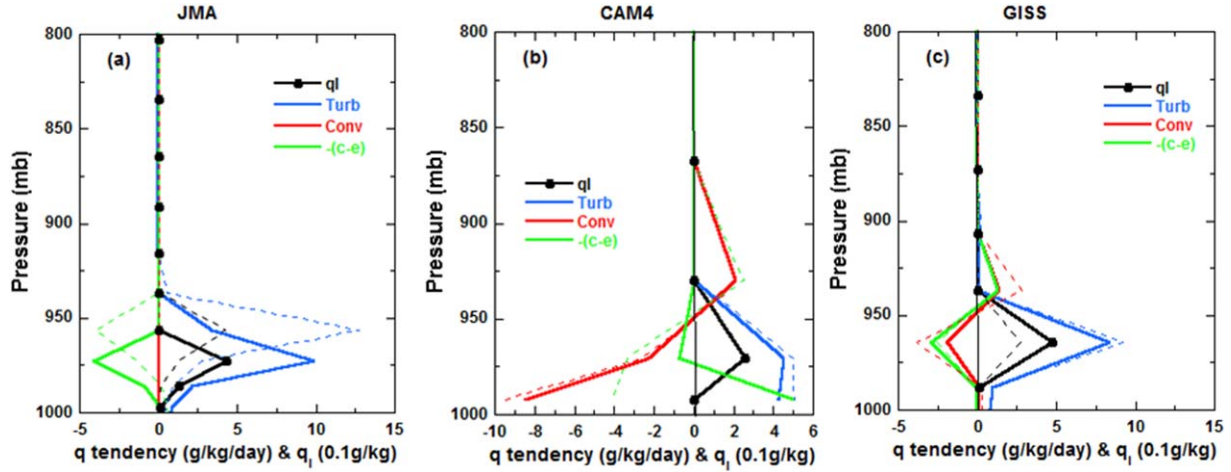
Figure 6. Solid lines are physical tendencies of water vapor (g/kg/day) in three SCMs at S11 for the control climate, “ turb ” for turbulence scheme, “ conv ” for convection scheme, “ (c-e) ” for net large-scale condensation, and “ ql ” for the grid-box cloud liquid water (0.1 g/kg). The black dots show the midpoint of model layers. The dashed lines show the corresponding values in the warmer climate. (a) JMA, (b) CAM4, and (c) GISS.
