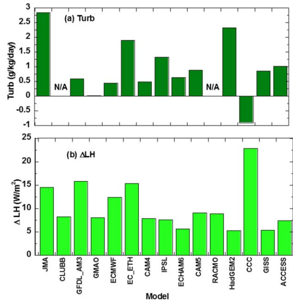
Figure 8. (a) Change of moisture tendency in the layer of maximum cloud water ( \text{g/kg/day} ) by the “Turb” term from the control climate to the perturbed climate at S11. (b) Same as Figure 8a but for surface latent heat flux ( \text{W/m}^2 ).
