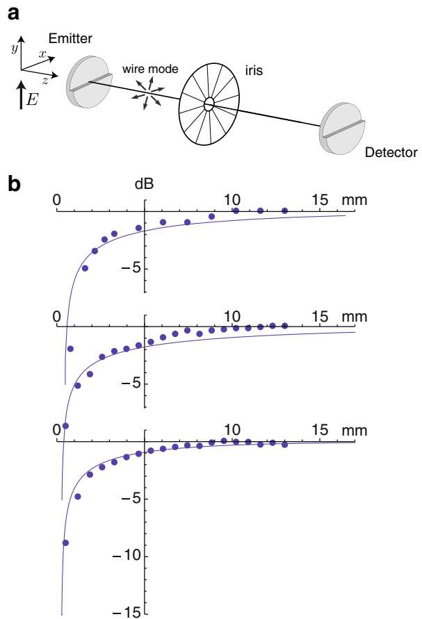
Fig. 3 (a) Schematic of the transmission experiment of a Sommerfeld mode on a wire of radius a with an iris as a variable attenuator. (b) Measured (dots) and calculated (solid lines) power transmissions as a function of the iris opening radius. Abscissa origin is taken at the wire center. Upper curve: stainless steel a = 400 \mu\text{m} f = 100 \text{ GHz} . Middle curve: tungsten a = 250 \mu\text{m} f = 100 \text{ GHz} . Lower curve: tungsten a = 250 \mu\text{m} f = 300 \text{ GHz} .
