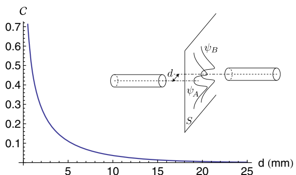
Fig. 2 Calculated coupling efficiency C between the ends of two tungsten wires of radius a = 250 \mu\text{m} supporting Sommerfeld propagating modes at f = 100 \text{ GHz} and separated laterally by the distance d . The inset gives a schematic description of the system considered.
