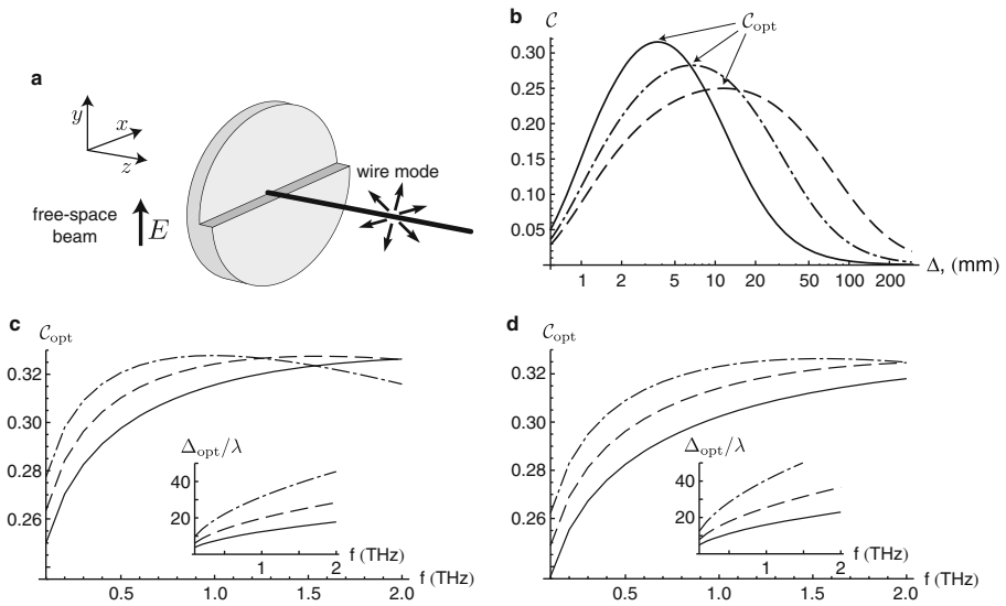
Fig. 1 Calculated coupling efficiency C between a linearly polarized gaussian beam of full-width at half power \Delta and a Sommerfeld mode propagating along a metal wire of radius a . (a) Schematic of the coupling scheme. (b) Coupling to a tungsten wire of radius a = 250 \mu\text{m} versus \Delta : f = 100 \text{ GHz} , dashed line; f = 300 \text{ GHz} , dot-dashed line; f = 1,000 \text{ GHz} , solid line. (c) Tungsten and (d) Gold: Maximum coupling efficiency, C_{\text{opt}} , as a function of frequency for various wire radius: a = 250 \mu\text{m} , solid line; a = 500 \mu\text{m} , dashed line; a = 1 \text{ mm} , dot-dashed line. Insets give the ratio of \Delta_{\text{opt}} to the wavelength, \Delta_{\text{opt}} being the beam width that achieves the maximum coupling efficiency C_{\text{opt}} .
