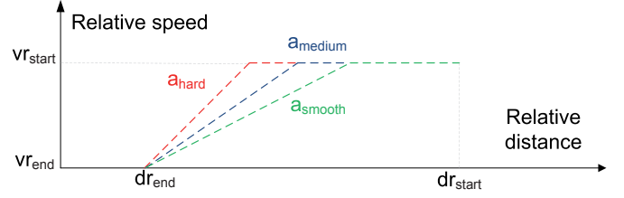
Fig. 6. Gap closing controller operation
