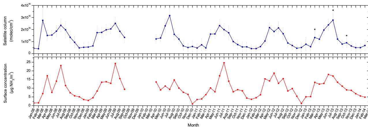
Figure 4. Time series of monthly averaged NH 3 satellite columns (top, blue, molec cm -2 ) and ground-based concentrations (bottom, red, \mu\text{g m}^{-3} ) at Shangzhuang site (40.14° N, 116.18° E) in the North China Plain (NCP) from January 2008 to February 2014. The associated weighted mean error for each month is calculated following equations described in Van Damme et al. (2014a) and presented here as error bars. Asterisks highlight the fertilization peaks of March, July and October 2013 (Shen et al., 2011).
