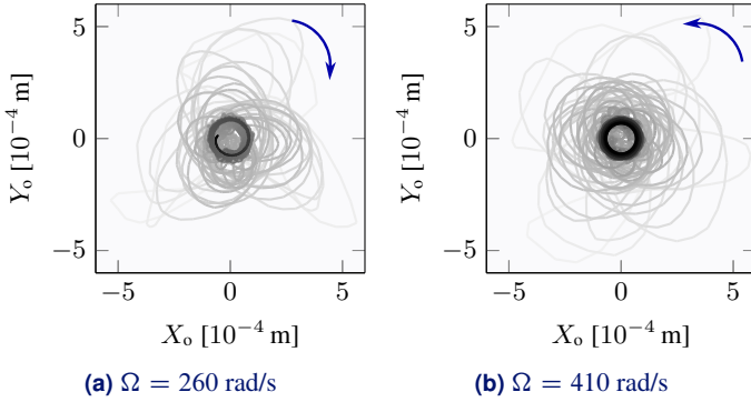
(a) \Omega = 260 rad/s (b) \Omega = 410 rad/s Figure 11. Center node displacements: sustained regime - transitory [—] and steady-state [—] response
