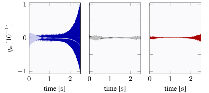
(a) k = 0 [—] and 1 [—] (b) k = 2 to 11 (c) susp. modes Figure 14. Modal contributions: \Omega = 420 rad/s
