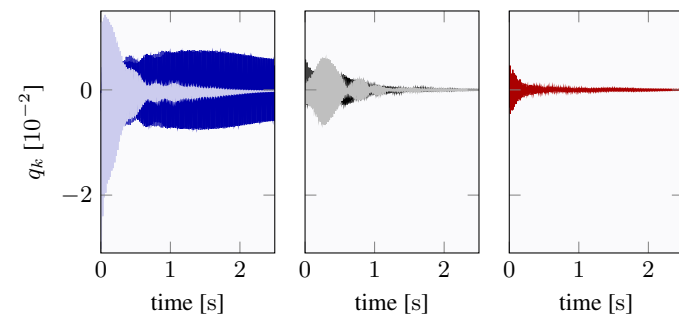
(a) k = 0 [—] and 1 [—] (b) k = 2 to 11 (c) susp. modes Figure 12. Modal contributions: \Omega = 410 rad/s
