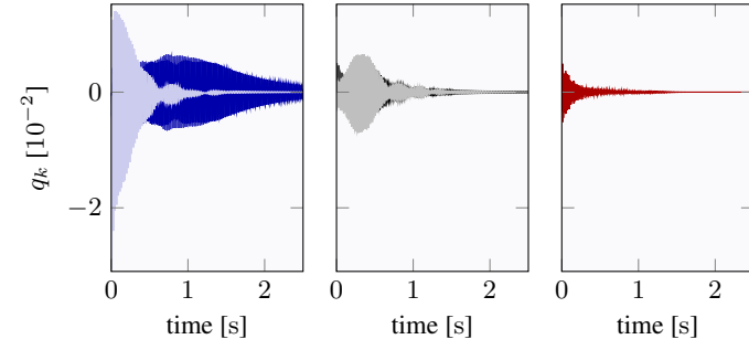
(a) k = 0 [—] and 1 [—] (b) k = 2 to 11 (c) susp. modes Figure 10. Modal contributions: \Omega = 520 rad/s
