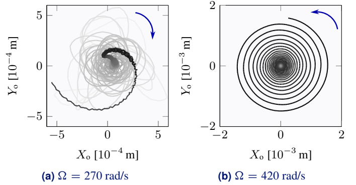
(a) \Omega = 270 rad/s (b) \Omega = 420 rad/s Figure 13. Center node displacements: divergent regime - transitory [—] and divergent [—] response
