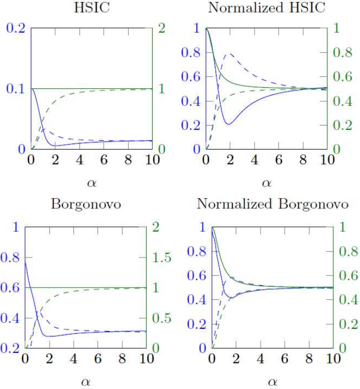
Figure 2: Standard and normalized HSIC and Borgonovo indices (blue lines) of X_1 (plain lines) and X_2 (dashed lines) for different values of \alpha , with the corresponding total Sobol' indices (green lines).
