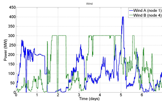
Figure 6: Wind power in production nodes for a typical week.
