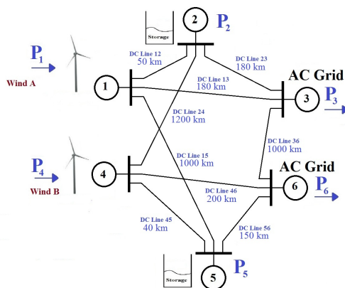
Figure 5: Six-terminal simulation grid.
