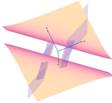
Figure 3: Intersection of hyperbolic cylinders.
