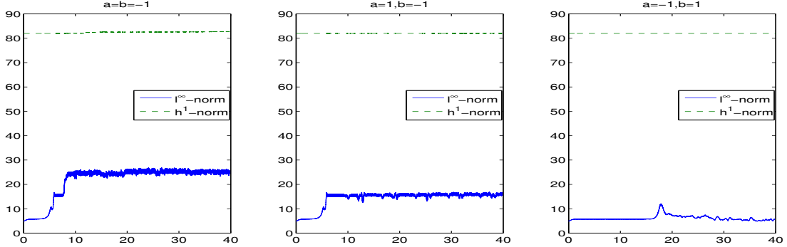
Figure 8: Evolutions of the h^1 -norm (---) and the l^\infty -norm (—) with respect to time. Here p = 2 , a = b = -1 , ab = -1 , c = 4 , K = 50 , L = M = 4 , N_x = 256 , N_y = N_z = 16 , \Delta t = 5 \times 10^{-4} , \lambda_y = 0.01 , \lambda_z = 50 and \varepsilon = 10^{-2} .
