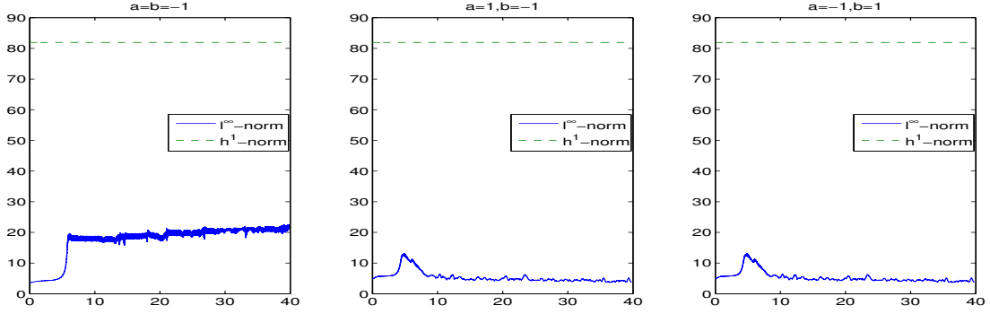
Figure 7: Evolutions of the h^1 -norm (---) and the l^\infty -norm (—) with respect to time for p = 2 , a = b = -1 , ab = -1 , c = 4 , K = 50 , L = M = 4 , N_x = 256 , N_y = N_z = 16 , \Delta t = 5 \times 10^{-4} , \lambda_y = \lambda_z = 50 and \varepsilon = 10^{-2} .
