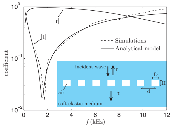
FIG. 1: Comparison between Eq. (1b) and simulation data extracted from figure 16 in Hladky-Henion et al. [20], for the transmission coefficient through a layer of air cylinders ( H = 2 cm, D = 1.5 cm) on a square lattice ( d = 5 cm) in silicone.
