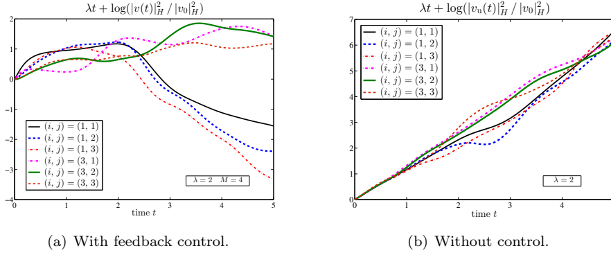
FIG. 2. Convergence rate is achieved with the feedback control.
