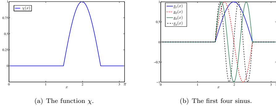
FIG. 1. Basis for the control space \{\chi \mathbb{E}_0^\mathcal{O} \eta \mid \eta \in \text{span}\{s_i \mid i \in \{1, 2, 3, 4\}\}\} .
