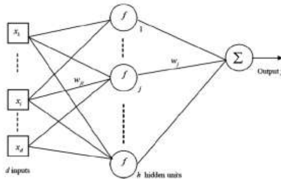
Fig. 1. Sketch of a MLP with d inputs and h hidden units, in our case, d=2 (clear sky index and \cos(SZA) ). The output y is the modeled bias correction.
