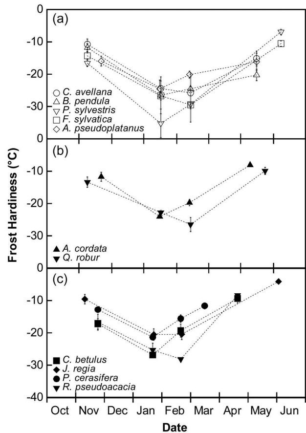
Figure 1. Seasonal change in frost hardiness (°C) of tree species according to their altitudinal distribution: high-mountain and sub-mountain species (a), low-mountain species (b) and lowland species (c). Symbols and bars represent mean and standard errors of three replicates.
