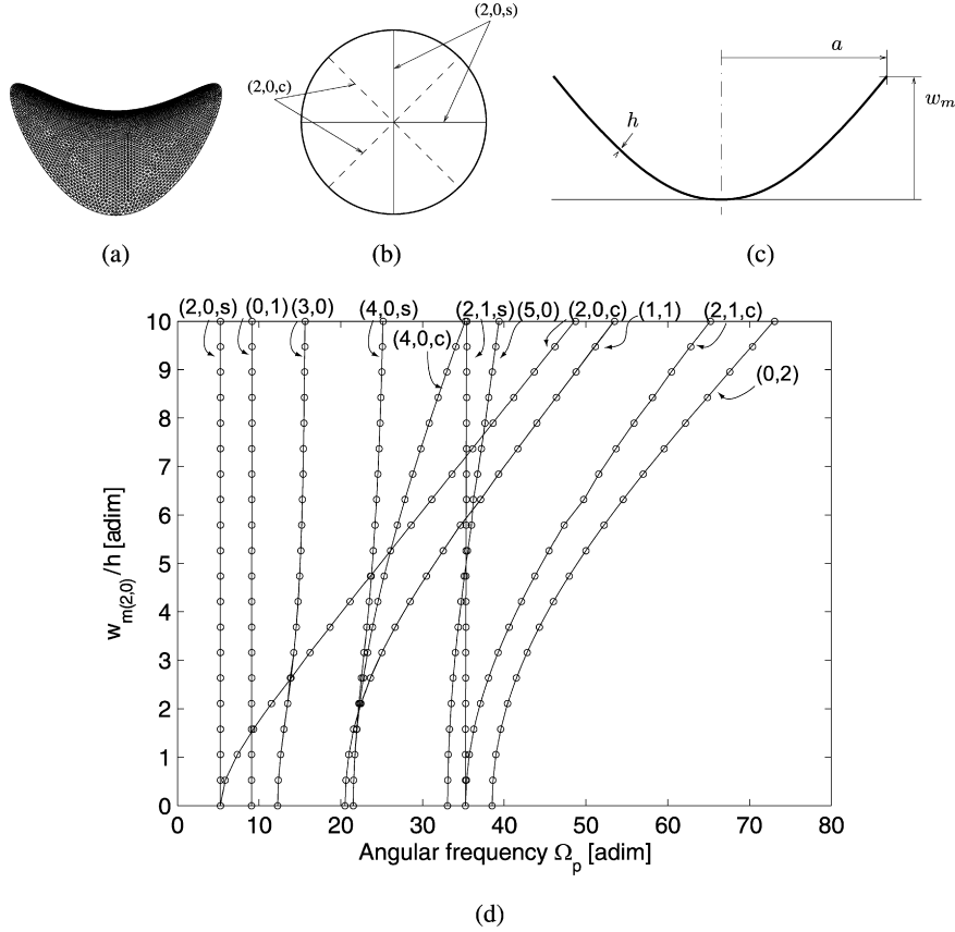
Fig. 8. (a) Finite element mesh, (b) top view with nodal radii of each configuration, (c) cross-section view of the imperfection having the shape of mode (2, 0, c). (d) Evolution of natural angular frequencies of the imperfect plate having the shape of mode (2, 0, c) with respect to the amplitude w_m of the imperfection normalized by h , according to CAST3M (—) and calculated from the present model (---).
