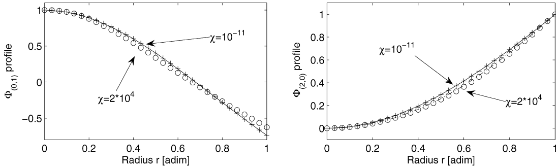
Fig. 3. Profiles of (0, 1) and (2, 0) mode shape for \chi = 10^{-11} and \chi = 2 \times 10^4 ; according to the spherical shell model (Thomas et al., 2005b) ((—) and (---)), and to the present model ((+) and (o)).
