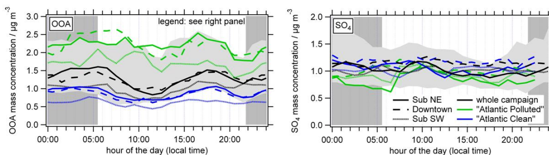
Fig. 6. Diurnal cycles (hourly median values) for OOA (left) and SO 4 (right) at all sites for the whole campaign, and for “Atlantic Polluted” and “Atlantic Clean” air masses separately. The time period between sunset and sunrise is shaded in grey. Percentiles (25 and 75 %) are shown in light grey exemplarily for the measurements at Sub NE only (whole campaign).
