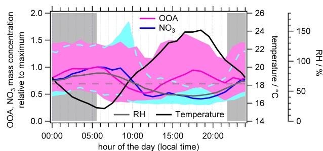
Fig. 7. Diurnal cycles (hourly median values) for the whole measurement campaign for the temperature and RH, and diurnal cycles for NO 3 and OOA, normalized to their respective maxima, all measured at Sub NE. Percentiles (25 and 75 %) are shown in light pink for OOA, and in light blue for NO 3 . The time period between sunset and sunrise is shaded in grey. Deliquescence RH for NH 4 NO 3 of 62 % (for 20 °C; Seinfeld and Pandis, 2006) for the transition of the solid to the liquid phase is marked as a dashed horizontal line.
