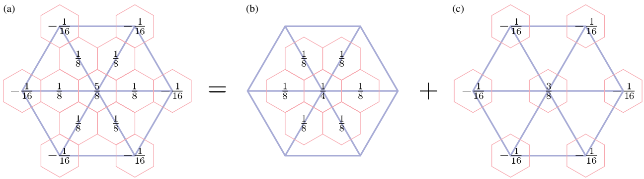
Figure 8. Decomposition of (a) the pressure restriction operator R_p^j into a sum of (b) an area-weighted restriction operator R_0^j and (c) a remainder \delta R_p^j . The remainder is proportional to the seven-point Laplacian on the coarse grid. This figure is available in colour online at wileyonlinelibrary.com/journal/qj
