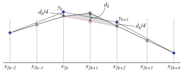
Figure 2. Lifted wavelet transform using linear interpolation. The thick line is the original signal on the fine grid and the thin line is the smooth signal on the coarse grid obtained by linear interpolation and lifting. The first stage in the smoothing (or restriction) is simply to neglect the odd points x_{2k+1} . The wavelet coefficient \tilde{x}_m is then the difference between the actual signal value x_{2k+1} and the value predicted by linear interpolation (indicated by the open red circle). In order to retain the moving average of the signal, the coarse grid values x_{2k} and x_{2k+2} are lifted by adding \tilde{x}_m/4 to obtain the coarse values y_k and y_{k+1} . (Figure adapted from Daubechies and Sweldens, 1998). This figure is available in colour online at wileyonlinelibrary.com/journal/qj
