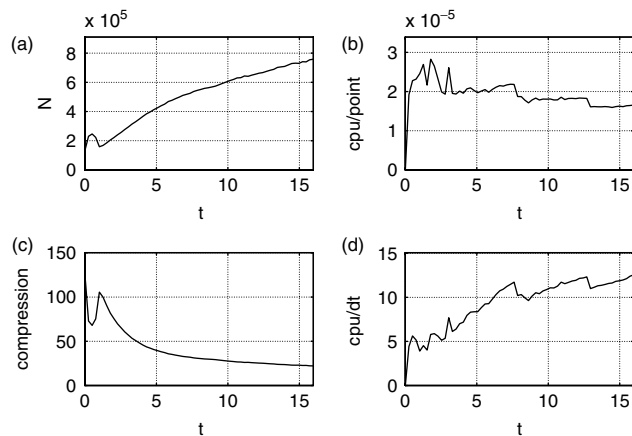
Figure 20. Compression properties of nonlinear inertia–gravity wave computation. The compression decreases as the wave packet steepens and broadens, but the cpu time per active point is approximately constant.
