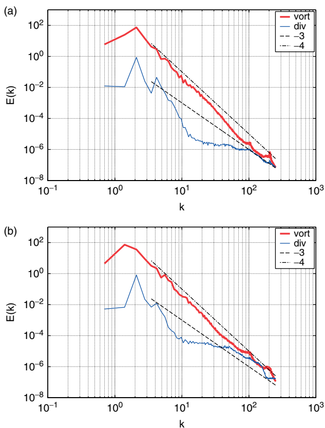
Figure 24. Vortical and divergent parts of the energy spectrum for the decaying shallow-water turbulence simulations with tolerances (a) \varepsilon = 0.15 at t = 25.03 , and (b) \varepsilon = 0.30 at t = 21.80 . Note that the vortical part of the two spectra are very similar, while the divergent part of the \varepsilon = 0.15 spectrum has less energy at intermediate and small scales. This figure is available in colour online at wileyonlinelibrary.com/journal/qj
