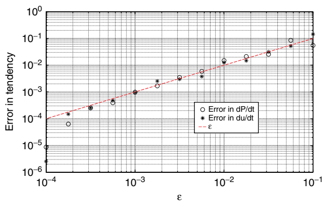
Figure 15. Control of tendency error in the inertia–gravity wave regime. The thresholds for pressure and velocity are respectively \varepsilon_p = c U \varepsilon^{3/2} and \varepsilon_u = U \varepsilon^{3/2} , to ensure that the error in the tendencies \partial_t p and \partial_t \mathbf{u} is O(\varepsilon) . This figure is available in colour online at wileyonlinelibrary.com/journal/qj
