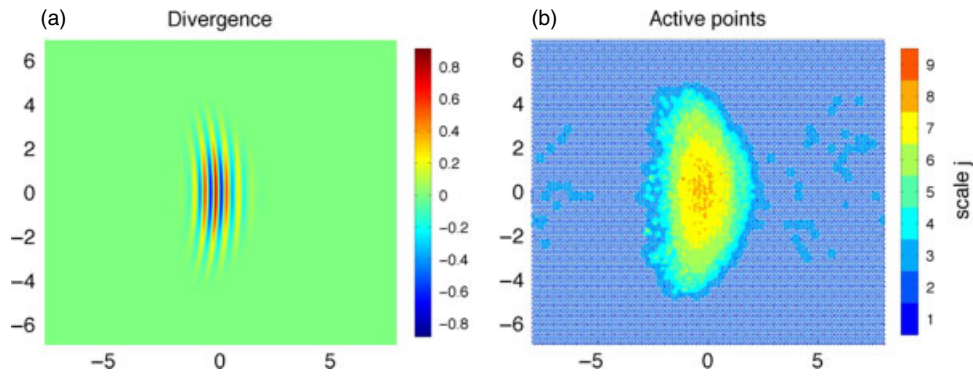
Figure 18. (a) Velocity divergence and (b) active wavelets for the linear inertia–gravity wave at t = 16 (one orbit of periodic domain). Note that the grid has tracked the advection and spreading of the wavefront. This figure is available in colour online at wileyonlinelibrary.com/journal/qj
