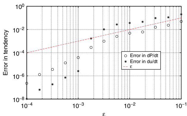
Figure 16. Control of the tendency error in quasi-geostrophic regime. The thresholds for pressure and velocity are respectively \varepsilon_p = Ro U f L \varepsilon^{3/2} and \varepsilon_u = Ro U L \varepsilon^{3/2} , to ensure that the relative error in the tendencies \partial_t p and \partial_t \mathbf{u} is O(\varepsilon) . The error decreases more rapidly for \varepsilon \leq 10^{-3} because the maximum allowable refinement level j = 12 has been reached. This figure is available in colour online at wileyonlinelibrary.com/journal/qj
