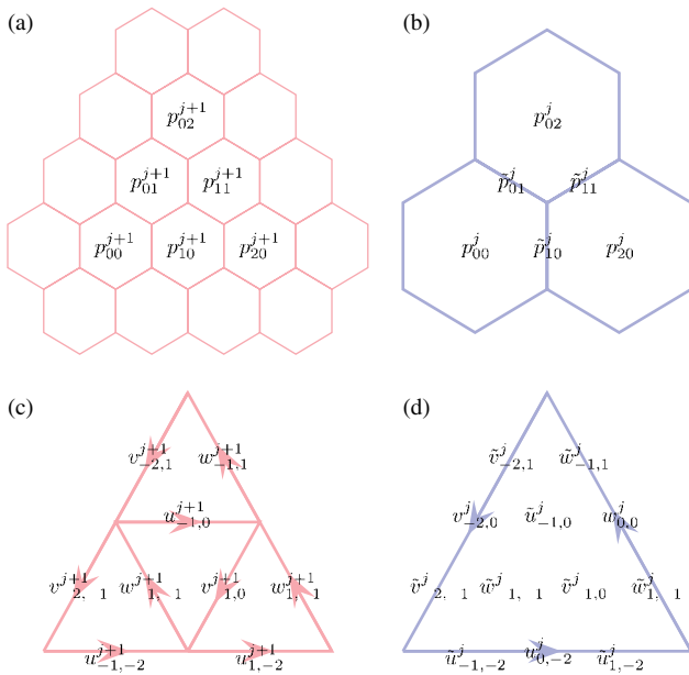
Figure 3. Arrangement of scaling function and wavelet coefficients on the multiscale triangular–hexagonal C-grid. (a, b): pressure on the hexagonal grid. (c, d): velocity on the triangular grid. (a, c): scaling function coefficients at the fine scale j + 1 . (b, d): scaling function and wavelet coefficients at the coarse scale j . The coarse scaling function coefficients p^j and u^j, v^j, w^j are smoothed versions of the pressure and velocity respectively. The wavelet coefficients are the difference between the exact value on the fine grid and the value interpolated from the coarse grid using the coarse scaling function coefficients. On each coarse triangular edge, the two velocity wavelet coefficients are equal and opposite, e.g. \tilde{u}_{-1,-2}^j + \tilde{u}_{1,-2}^j = 0 . This figure is available in colour online at wileyonlinelibrary.com/journal/qj
