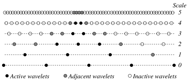
Figure 11. One-dimensional example showing adjacent wavelets in position and scale that are added to the grid of active wavelets to account for the change in the solution over one time step.
