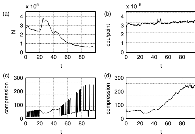
Figure 23. Adaptive properties of the turbulence simulation with tolerance \varepsilon = 0.15 . (a) shows the total number of active points which is greatest when the turbulence is most intense (around t = 25 ). (b) shows that the computational cost per grid point is roughly constant, independent of the number of active points and the compression. (c) shows the compression based on the maximum active scale at any given time (and hence jumps when the maximum active scale changes), and (d) shows the compression rate measured based on the maximum allowable resolution (i.e. 2048^2 ).
