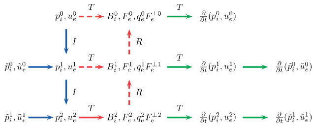
Figure 6. Conservative adaptive computation of the tendencies \partial_t \tilde{p}_m^j, \partial_t \tilde{u}_n^j, \partial_t p_i^j, \partial_t u_e^j from \tilde{p}_m^j, \tilde{u}_n^j, p_i^j and u_e^j . In the above method conservation of total mass is guaranteed. Blue arrows correspond to step 1 (synthesis, algorithm 2.2), red arrows to step 2 and green arrows to step 3. The interpolation, restriction and TRiSK operators are labeled as I, R and T respectively. Dashed arrows indicate that either restriction or TRiSK operators are used. In this minimal example the finest level is at j = 2 . Therefore the lowermost red T -arrow is solid as no data is available from level j + 1 to apply the restriction operators. Additional levels can be added by repeating the intermediate line j = 1 . This figure is available in colour online at wileyonlinelibrary.com/journal/qj
