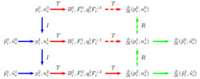
Figure 4. Non-conservative computation of the tendencies \partial_t \tilde{p}_m^j, \partial_t \tilde{u}_n^j, \partial_t p_i^j, \partial_t u_e^j from \tilde{p}_m^j, \tilde{u}_n^j, p_i^j and u_e^j . In the above method conservation of total mass is not guaranteed. Blue arrows correspond to step 1, red arrows to step 2 and green arrows to step 3. The interpolation, restriction and TRiSK operators are labeled as I, R and T respectively. Dashed arrows indicate that either restriction or TRiSK operators are used. In this minimal example the finest level is at j = 2 . Therefore the lowermost red T -arrow is solid as no data is available from level j + 1 to apply the restriction operators. Additional levels can be added by repeating the intermediate line j = 1 . This figure is available in colour online at wileyonlinelibrary.com/journal/qj
