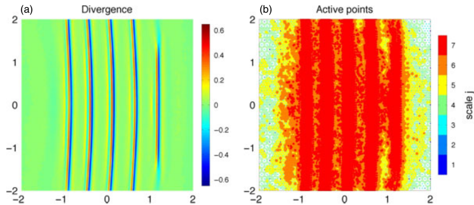
Figure 19. As Figure 18, but for the nonlinear wave and zoomed to show the small-scale structure. The grid has tracked the advection and steepening of the nonlinear wave. This figure is available in colour online at wileyonlinelibrary.com/journal/qj
