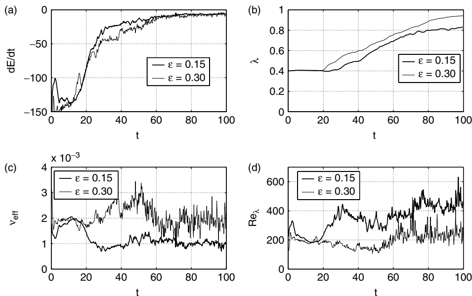
Figure 26. Dynamical quantities compared for turbulence simulations with tolerances \epsilon = 0.3 and \epsilon = 0.15 : (a) energy decay dE/dt , (b) Taylor scale \lambda , (c) the effective viscosity \nu_{\text{eff}} , and (d) the effective Taylor Reynolds number Re_\lambda . The effective Reynolds number appears to be roughly inversely proportional to the tolerance after the initial laminar period.
