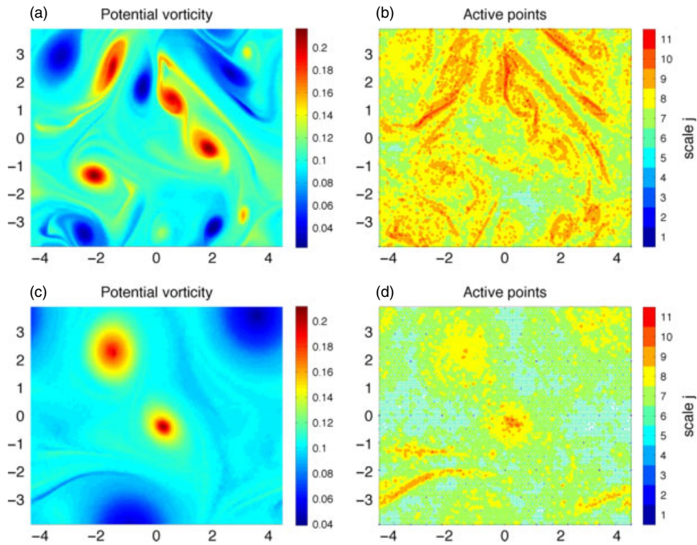
Figure 22. (a, c) Potential vorticity and (b, d) adapted grids for decaying quasi-geostrophic turbulence computed with tolerance \varepsilon = 0.15 at (a, b) an intermediate time ( t = 39.8 ) and (c, d) a late ( t = 74.8 ) time. This figure is available in colour online at wileyonlinelibrary.com/journal/qj
