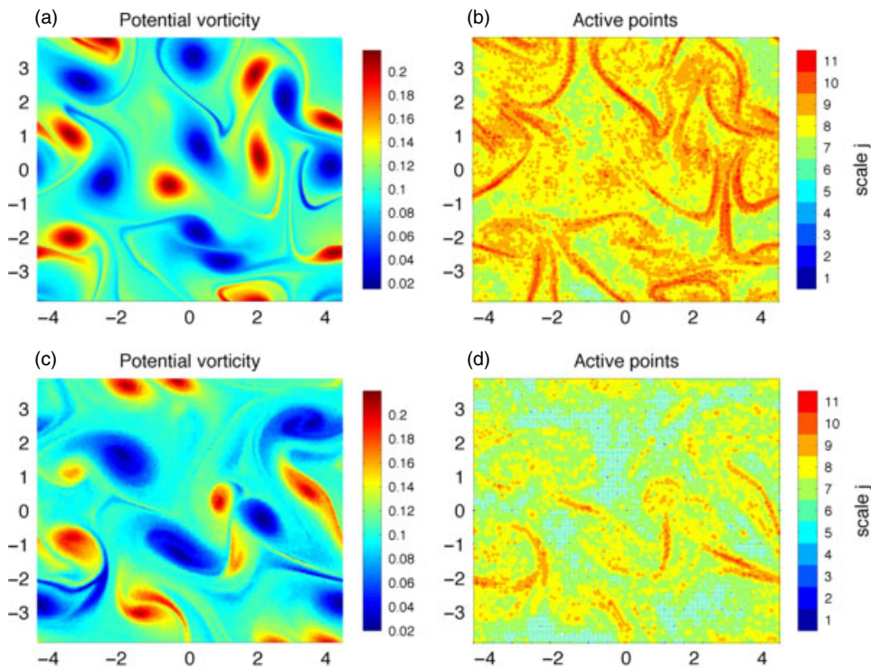
Figure 21. (a, c) Potential vorticity and (b, d) adapted grids for decaying quasi-geostrophic turbulence just after the turbulence is fully developed: (a, b) at t = 25.03 for tolerance \varepsilon = 0.15 , and (c, d) at t = 21.80 for tolerance \varepsilon = 0.30 . Two and three levels of refinement have been added, respectively, compared to the initial condition. There are significant coarse regions between the coherent structures and filaments. This figure is available in colour online at wileyonlinelibrary.com/journal/qj
