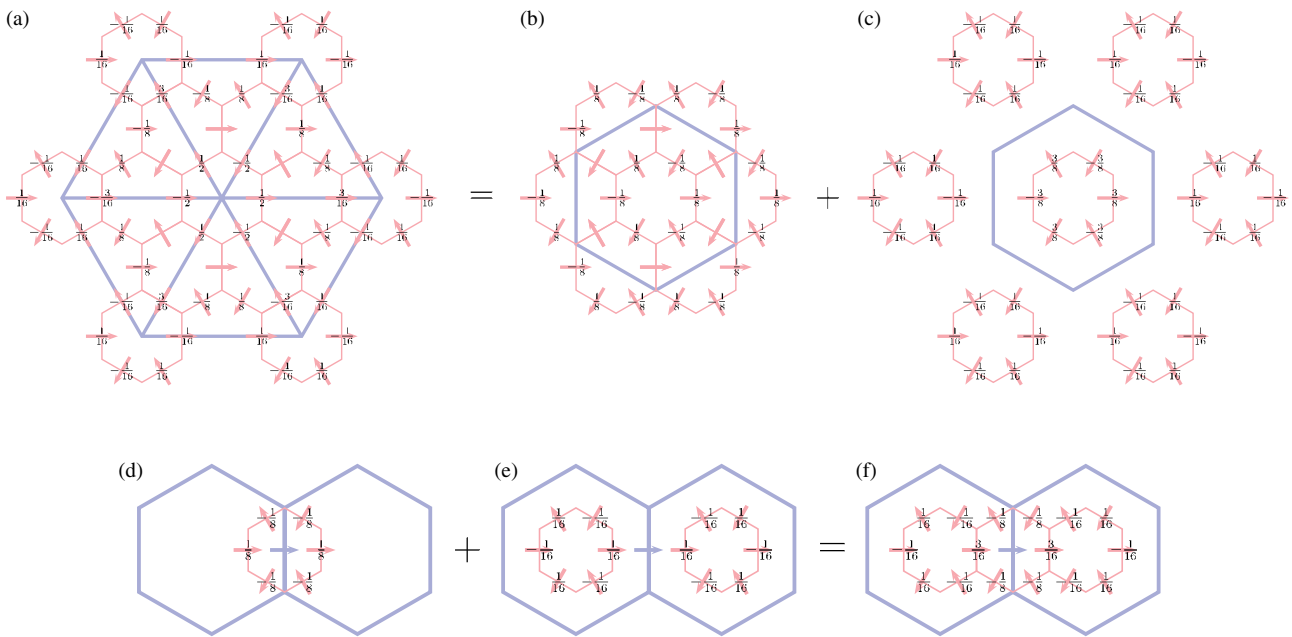
Figure 9. (a) Stencil of R_p^j \circ \text{div}^{j+1} (div operator followed by the pressure restriction operator) and its decomposition into (b, c) two simpler operators for which a compatible flux restriction operator can be found readily. (d) basic and (e) corrective flux restriction operators R_{0f}^j and D^j \circ \text{div}^{j+1} combined to give (f) the final mass flux restriction operator R_f^j , compatible with the mass restriction operator R_p^j and the div operators \text{div}^j, \text{div}^{j+1} in the sense of Figure 5. This figure is available in colour online at wileyonlinelibrary.com/journal/qj
