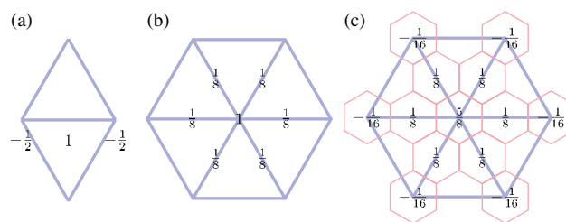
Figure 7. Stencils of the (a) interpolation, (b) lifting and (c) restriction operators for pressure. This figure is available in colour online at wileyonlinelibrary.com/journal/qj
