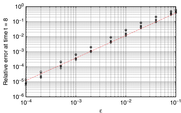
Figure 17. Accumulated time integration errors at t = 8 for the linear gravity wave case as a function of tolerance \varepsilon : L_1 error ( \circ ), L_2 error ( \square ), L_\infty error ( \diamond ). Errors in p are indicated by open symbols and errors in \mathbf{u} by filled symbols. The straight line shows a \varepsilon^{3/2} scaling. This figure is available in colour online at wileyonlinelibrary.com/journal/qj
