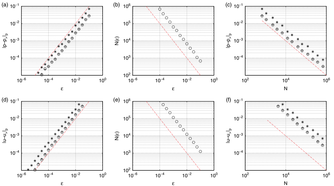
Figure 14. Control of error in (a, b, c) pressure and (d, e, f) velocity. \varepsilon is the threshold, and N(\varepsilon) is the number of active pressure or velocity wavelet coefficients. \circ denotes the L^1 error norm, + the L^2 error norm and * the L^\infty error norm. The straight lines give the theoretical scalings for second-order accurate interpolation in two dimensions (i.e. error \propto N^{-1} , and N \propto \varepsilon^{-1} ). Note that the most important property is that the error is proportional to (and hence controllable by) the threshold \varepsilon . This figure is available in colour online at wileyonlinelibrary.com/journal/qj
