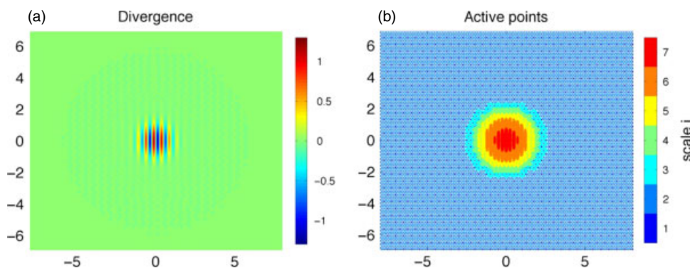
Figure 12. Initial conditions for the inertia–gravity wave case. The maximum allowable resolution is 2048^2 and the period cell has sides of length 16. (a) shows the velocity divergence and (b) the initial adapted grid (pressure and velocity wavelet points) used for the simulations. The tendency threshold is set to \varepsilon = 0.05 , corresponding to pressure and velocity thresholds \varepsilon_p = \varepsilon_u = 1.118 \times 10^{-3} . This figure is available in colour online at wileyonlinelibrary.com/journal/qj
