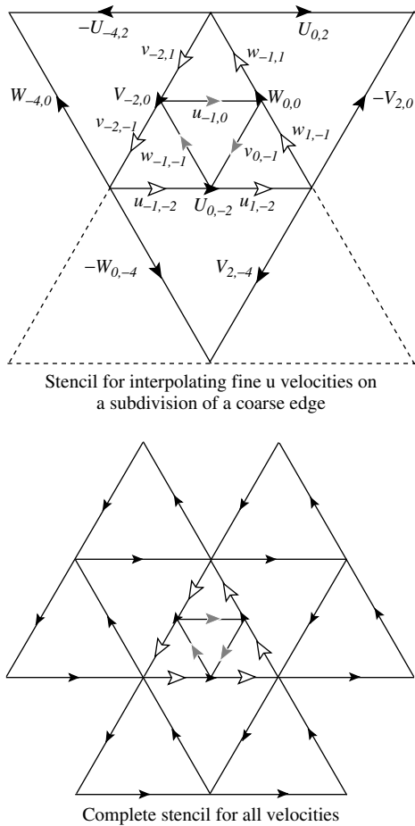
Figure 10. Stencil for circulation-conserving second-order interpolation of velocity (filled black arrows). Velocities on the bisection of coarse edges (unfilled black arrows) are obtained by linear interpolation. The velocities on inner fine triangle (grey arrows) are then obtained by assuming constant circulation over the coarse triangle. The dotted lines indicate the mirror-symmetric stencil. This stencil works for both valence 6 points (hexagon points) and valence 5 points (pentagon points) on subdivisions of the icosahedral sphere.
