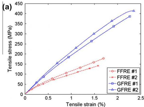
Fig. 2. Quasi-static responses in tensile loading of (a) [0/90]_{3S} and (b) [\pm 45]_{3S} for FFRE and GFRE specimens.
