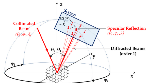
Figure 8: Illustration of the diffraction phenomenon by HCP structure at zero and first order diffraction on a screen.
